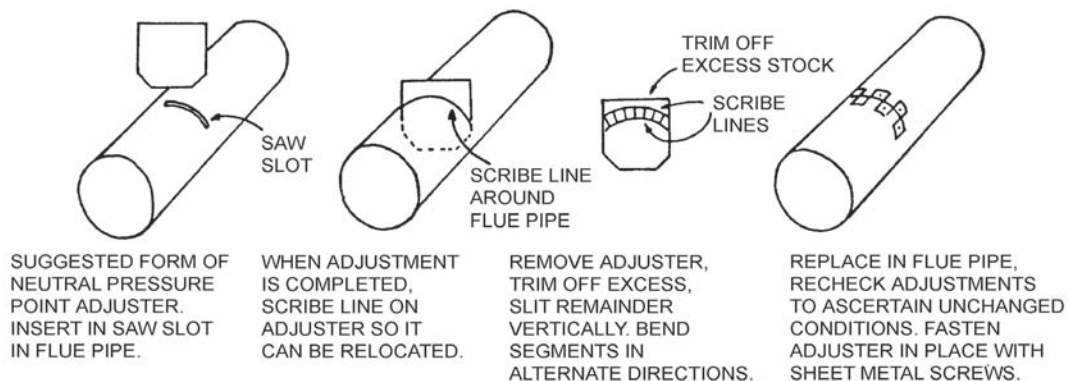
FIG. 3 – CONTROLLING EXCESSIVE DRAFT WITH A NEUTRAL PRESSURE POINT ADJUSTER
