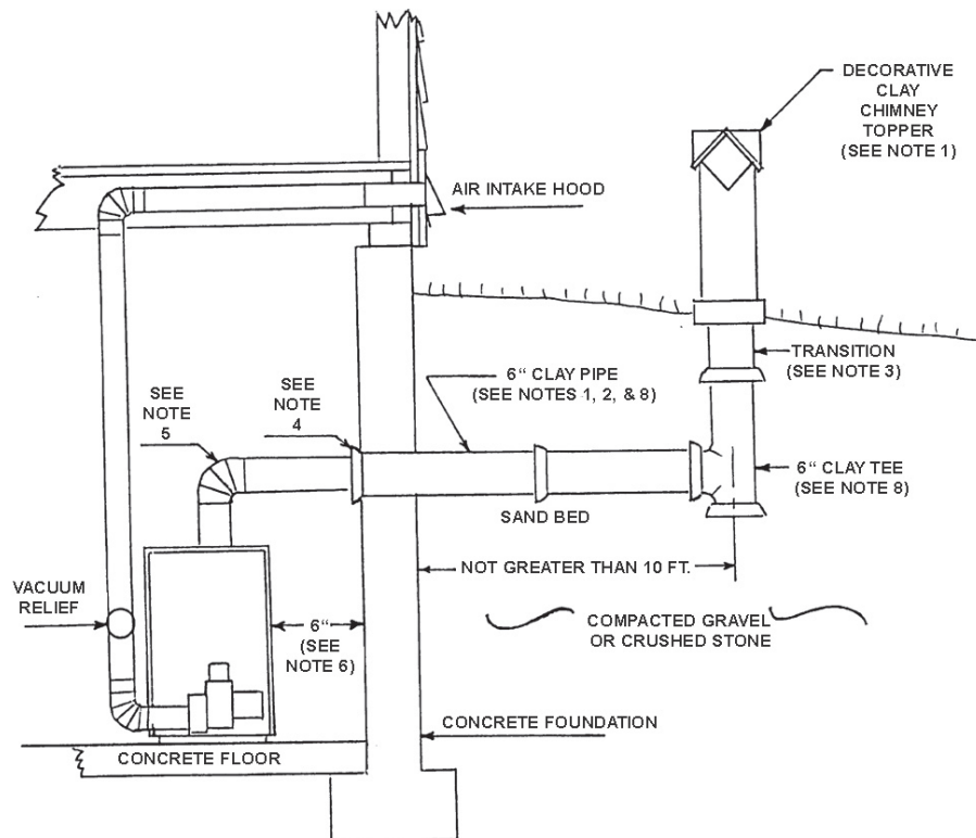
FIG. 6 – TYPICAL UNDERGROUND VENT INSTALLATION
