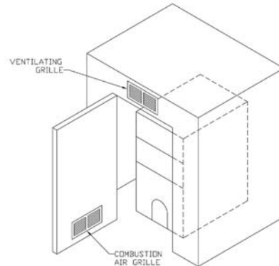
FIG. 1 – AIR OPENINGS FOR CLOSET OR UTILITY ROOM INSTALLATIONS
