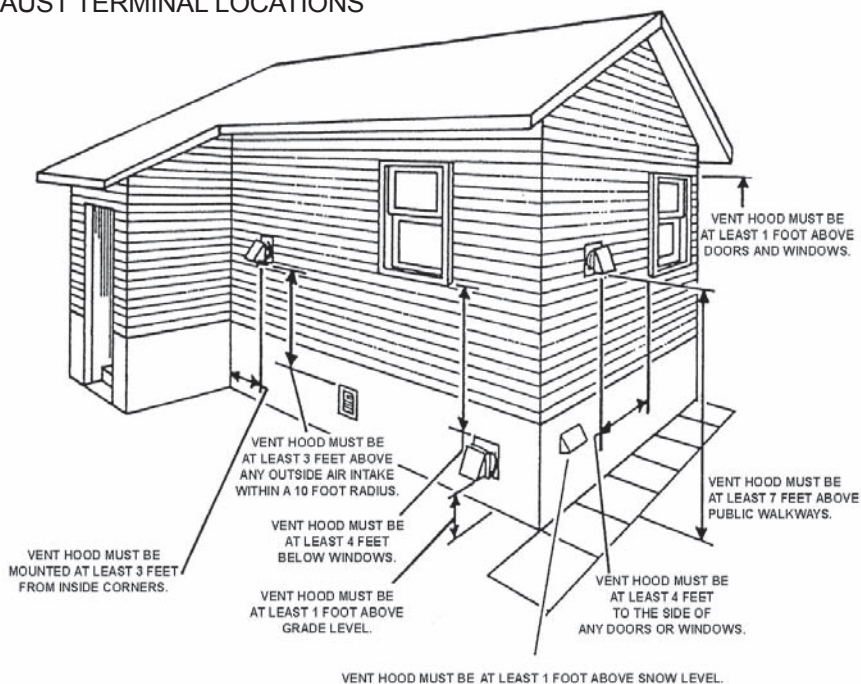
FIG. 5 – EXTERIOR EXHAUST TERMINAL LOCATIONS
