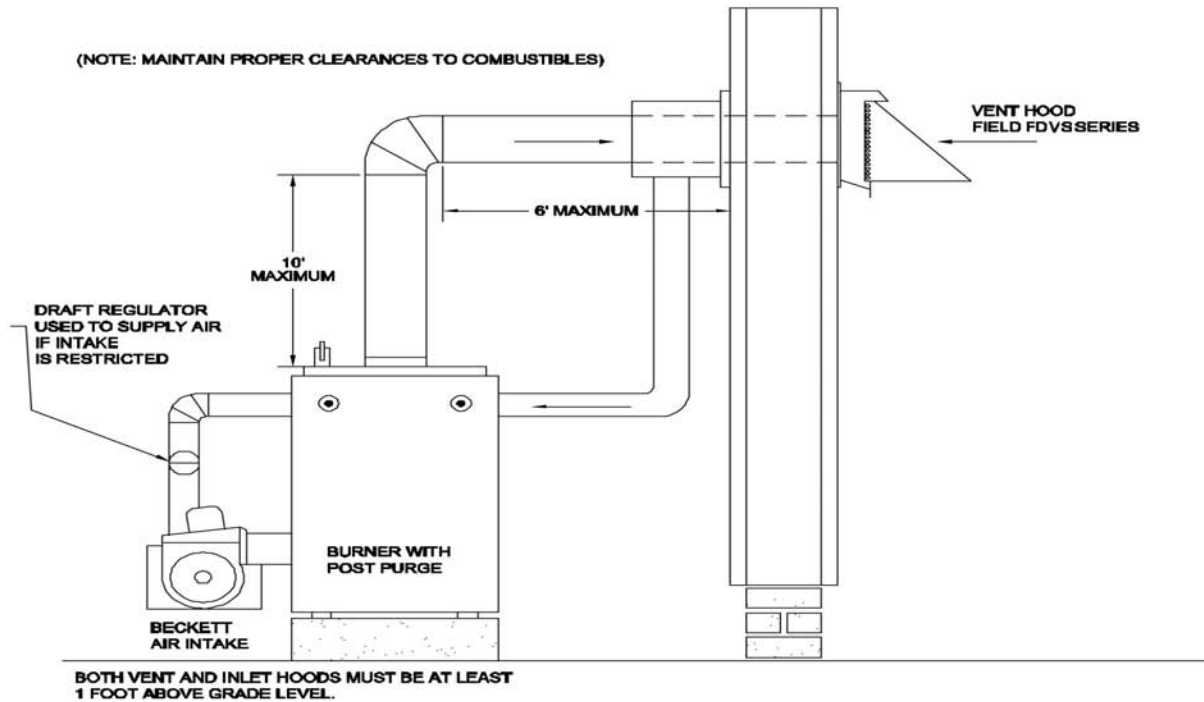
FIG. 4 – TYPICAL DIRECT EXHAUST INSTALLATION (W/BECKETT AFG OIL BURNER)
