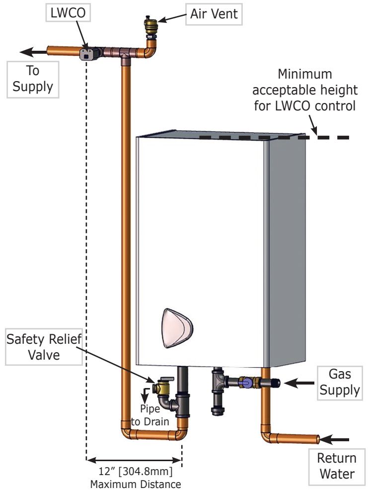
Figure 10 - LWCO Suggested Probe Location
