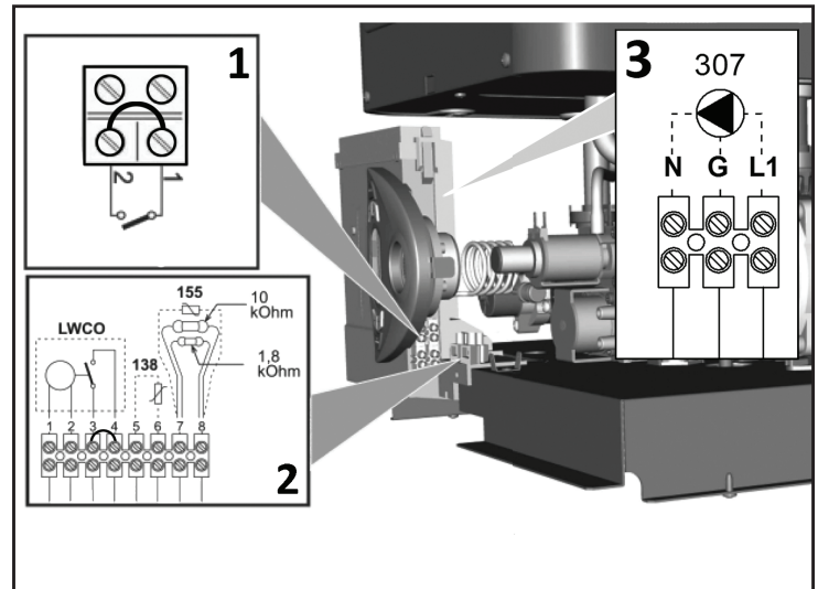
Figure 18 - Terminal Block
