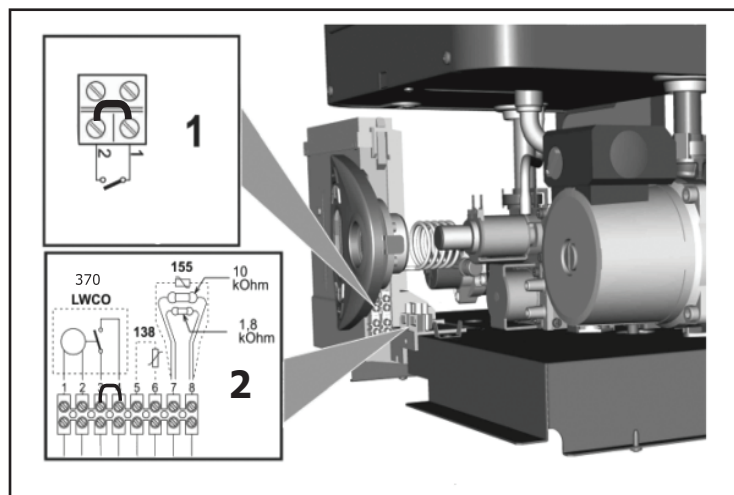
Figure 18 - Bornier
