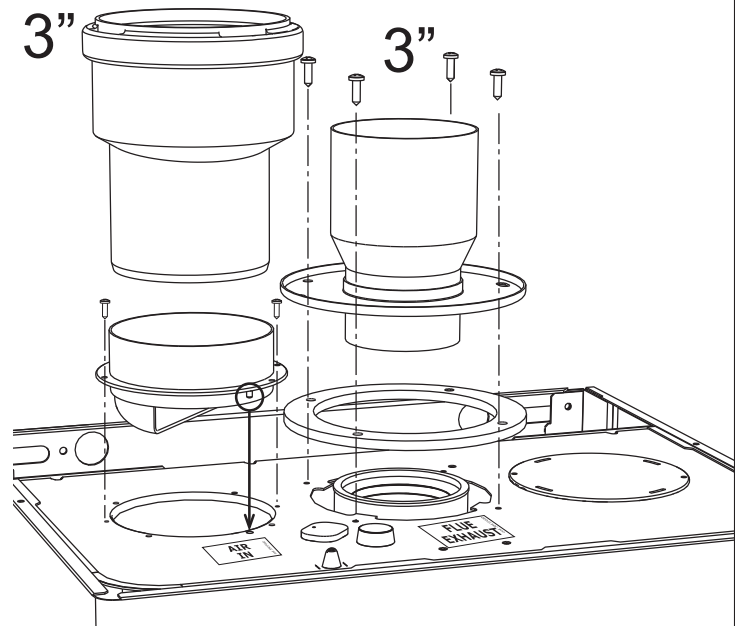
Figure 12 - Combustion Air Fitting
