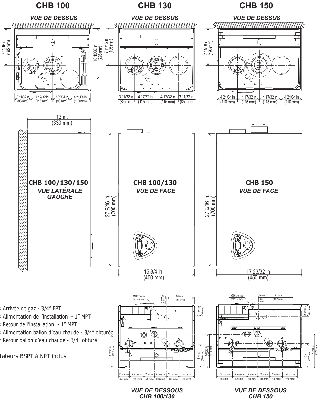
Figure 1 - Dimensions
