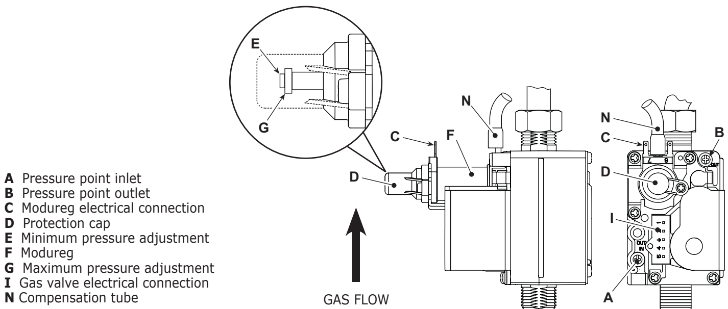
Figure 20 - Gas Valve
