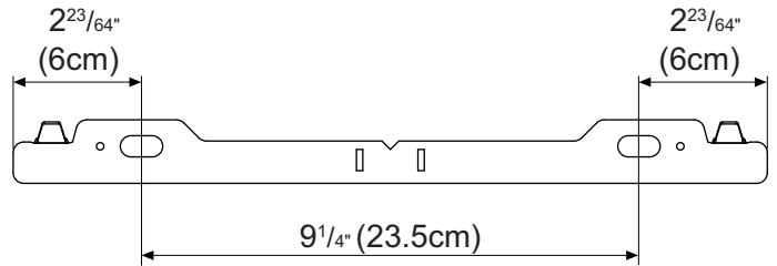
Figure 6 - Wall Mounting Bracket
