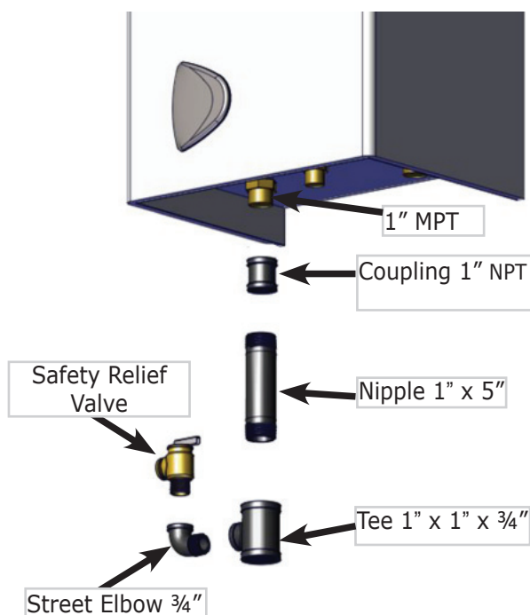
Figure 8 - Safety Relief Valve & Air Vent (Viewed from front of boiler)
