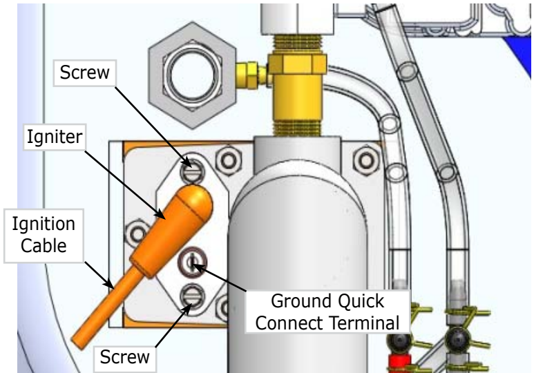
Figure 1 - Remove Ignitor (Procedure 2 To 4)
