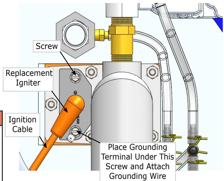
Figure 2 - Replace Ignitor (Procedure 5 To 9)
