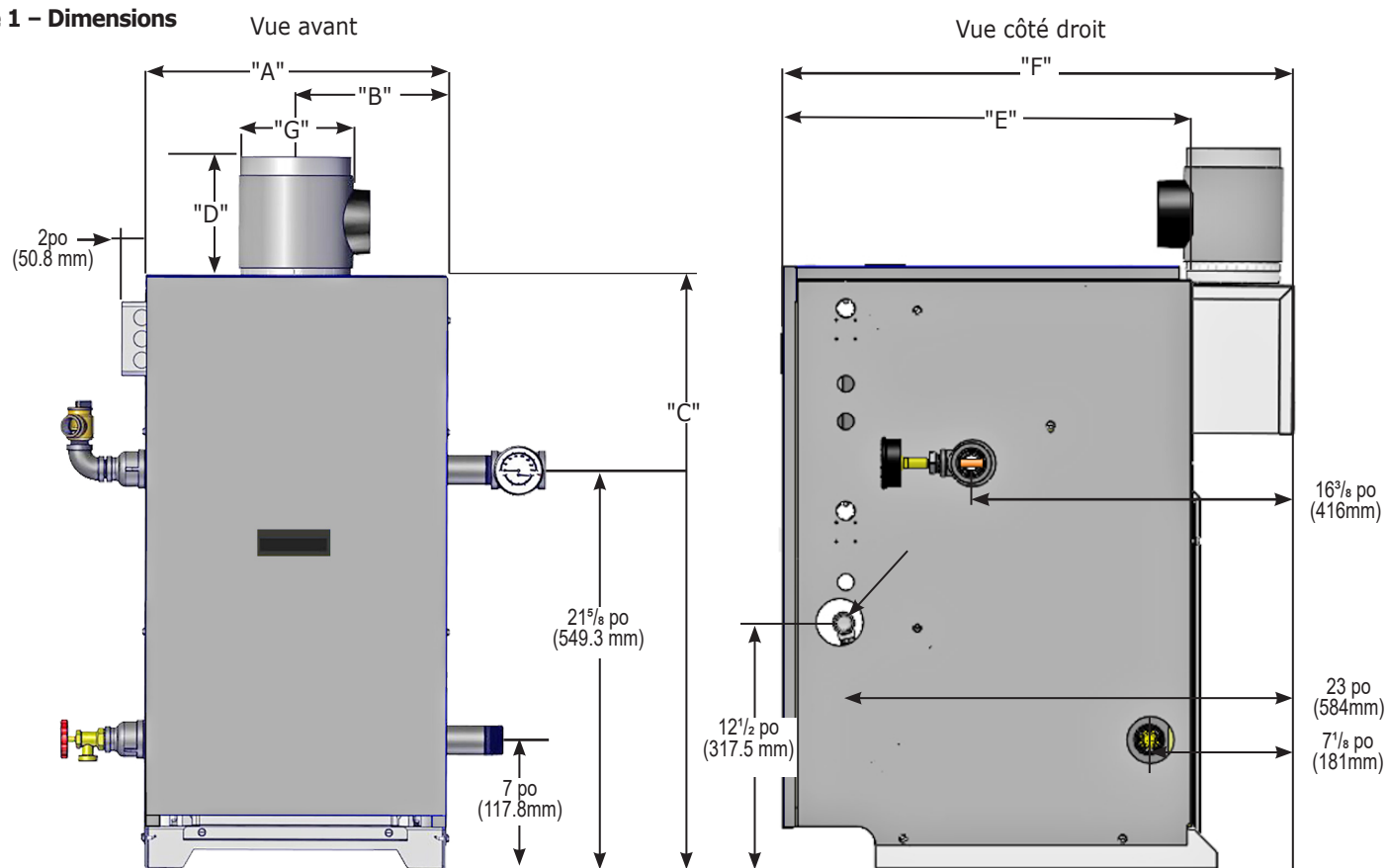
Figure 1 – Dimensions
