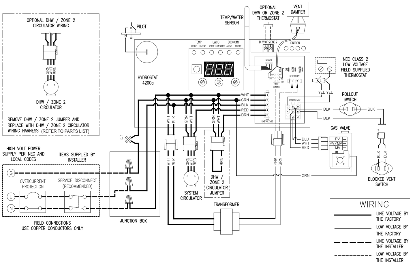
Figure 11-1 - 4200 Fuel Smart Hydrostat IC Control
