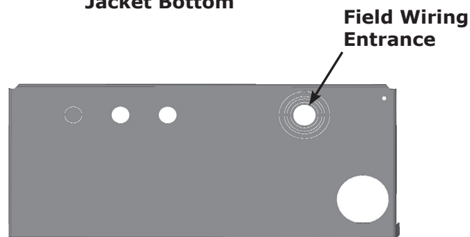
Figure 4 - Stepped Electrical Knock-outs - Jacket Bottom
