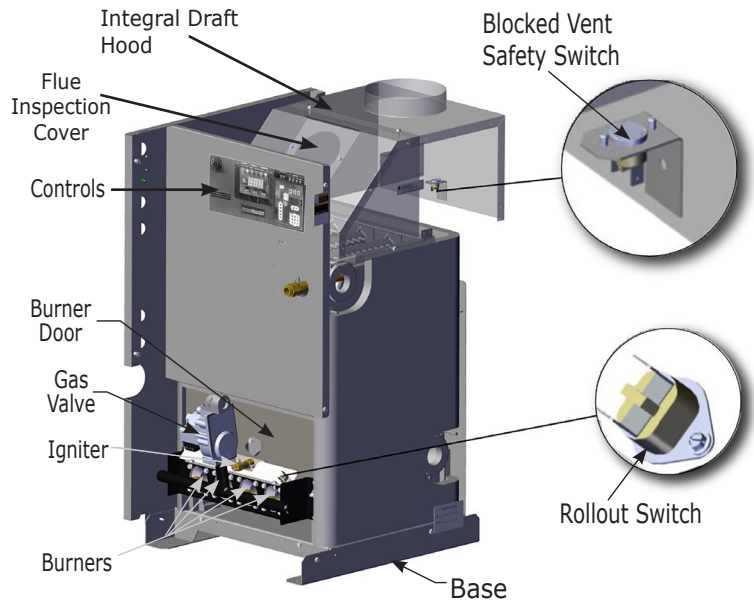
FIGURE 2 - BOILER FLUE GAS PASSAGEWAYS
