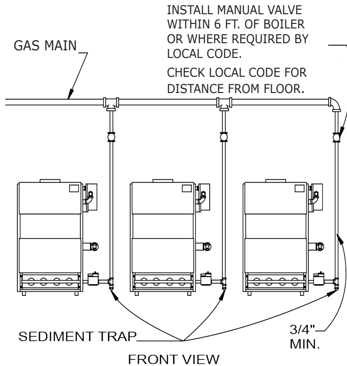
Figure 10 - Gas Piping - Modular Boilers
