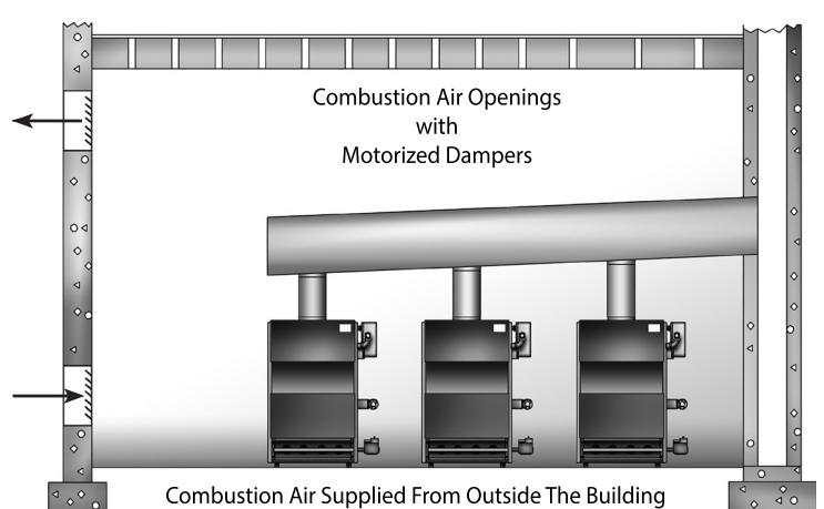
Figure 9 - Combustion Air with Motorized Dampers
