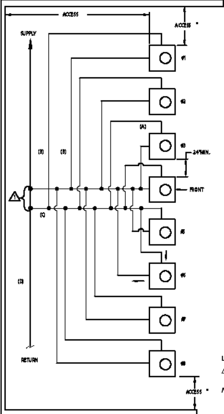
Figure 6 - Eight (8) Unit Configuration - Two Headers
