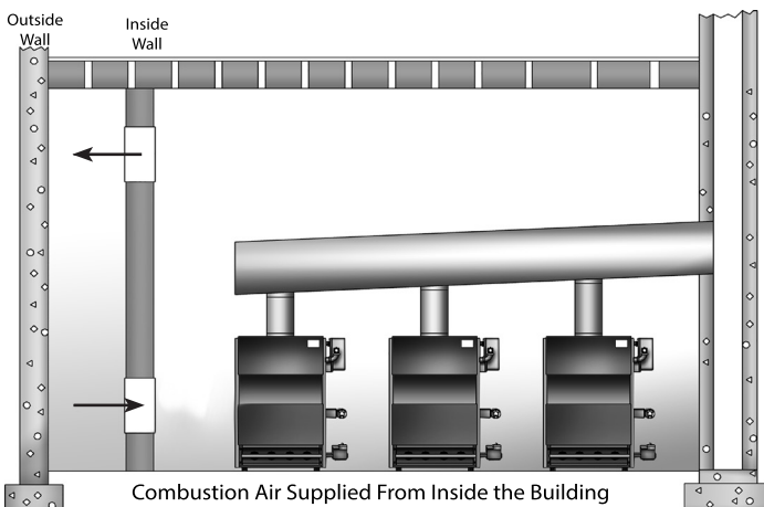
Figure 8 - Combustion Air Openings
