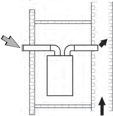
Figure 15 - Chimney Venting with Outside Air Single Wall
