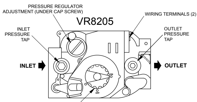
Figure 1 - Gas Valve Detail
